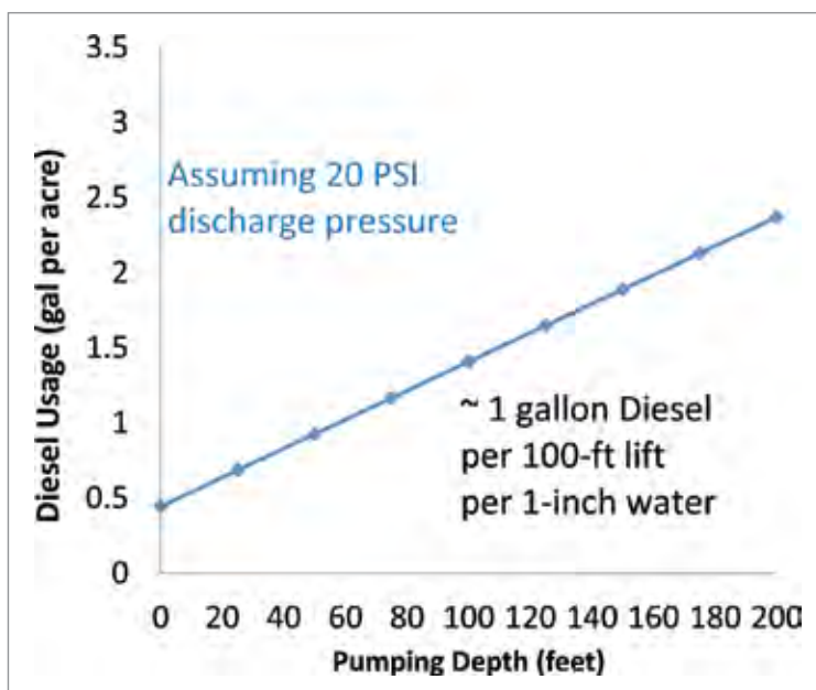
Figure 2.2 – Gallons of Diesel to apply 1 inch of water to one acre
