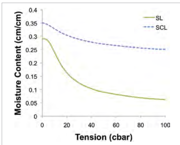
Figure 2.3 – Soil moisture release curves for sandy clay loam (SCL) and sandy loam (SL) soil types.
