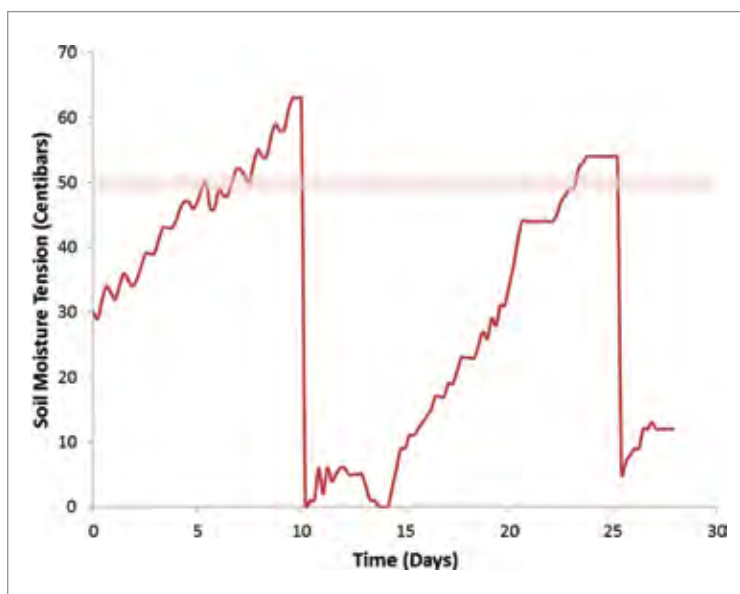
Figure 6.5 – Soil moisture tension versus time for Mississippi cotton in the early squaring growth stage (not a high water use time).
