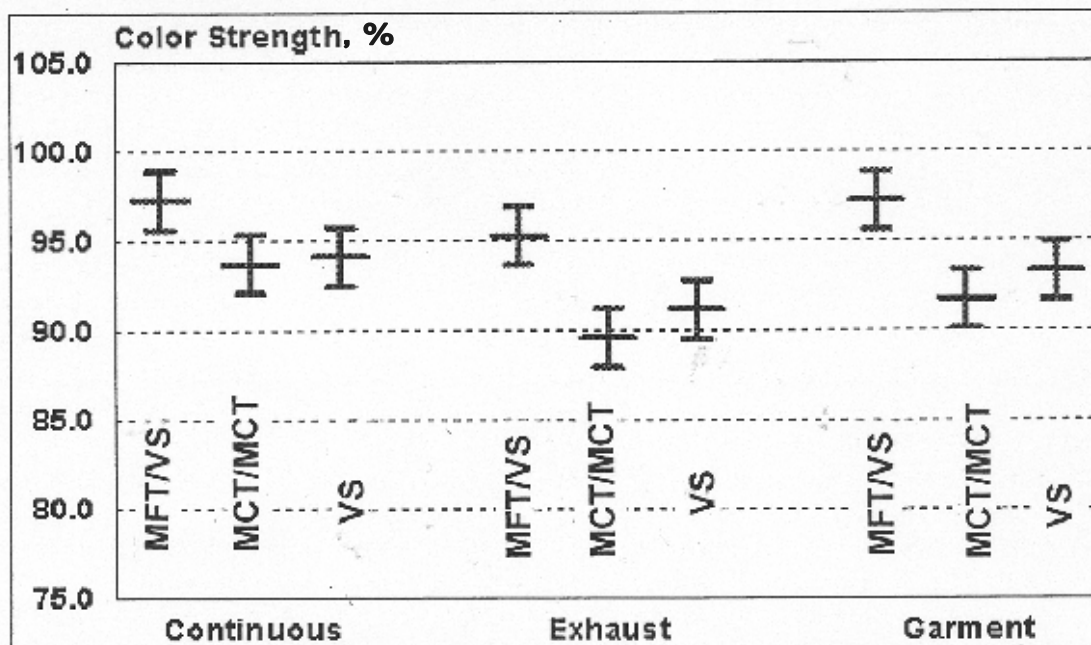
Figure 5. The effects of dyeing system and dyeing process on the color strength of the green shades finished with a conventional resin formula after 20 home laundry/tumble dry cycles.
