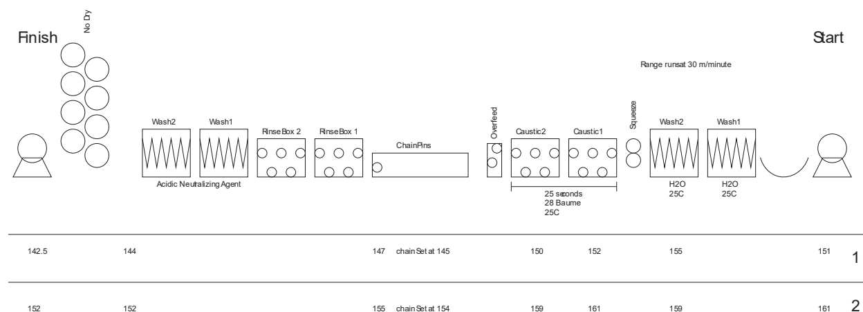
Figure 3 Example of Benninger Mercerizer with width readings (in cm) throughout process.
