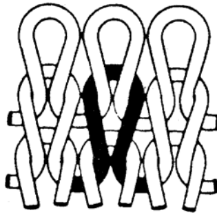
Figure 1 - Ideal alignment of course and wale loops. Wale loops are vertical and course loops are horizontal.
