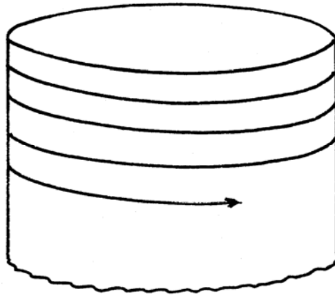
Figure 8 - Fabric course skew (spiral) for counterclockwise cylinder rotation. Fabric has a left hand skew.
