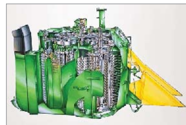
In-line row unit with both drums on the same side of the row.
