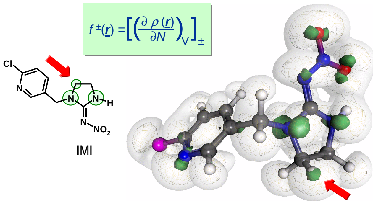
Figure 1. Isosurfaces of the Fukui function for electrophilic attack on IMI. Three levels of isosurfaces are displayed, 0.005 (green, opaque), 0.001 (yellow, transparent) and 0.0005 (white, transparent)
