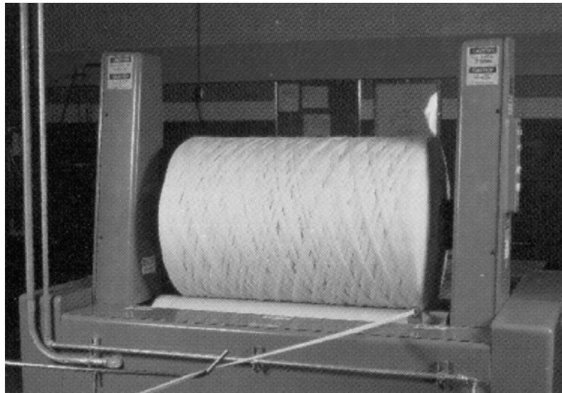
Figure 5. Ball Warping
