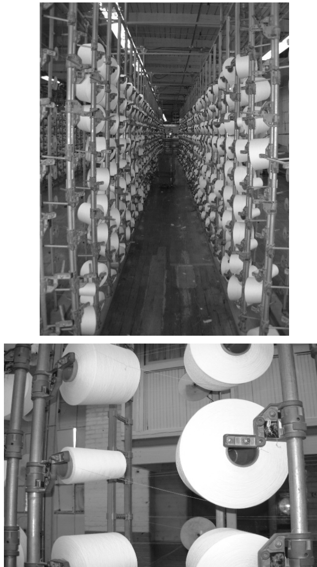
Figure 4. Magazine Creels
