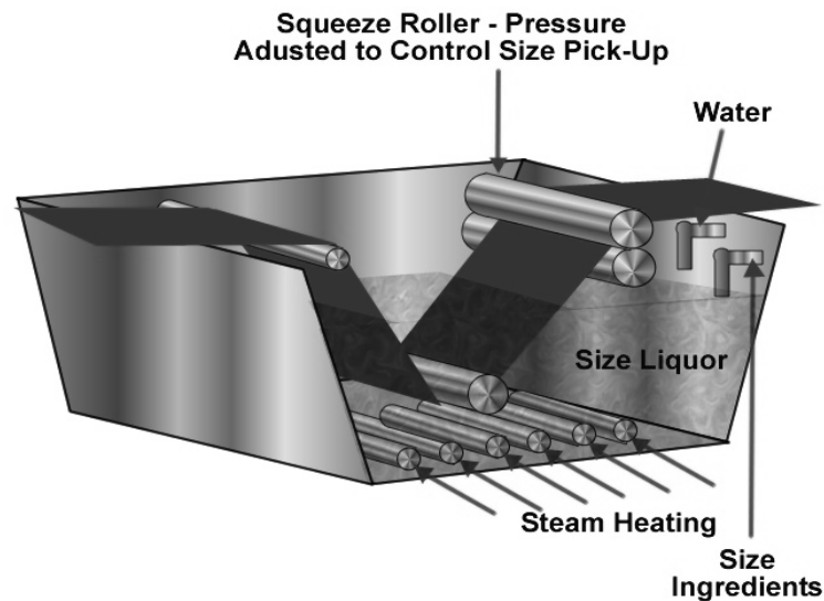
Figure 12. Size Box
