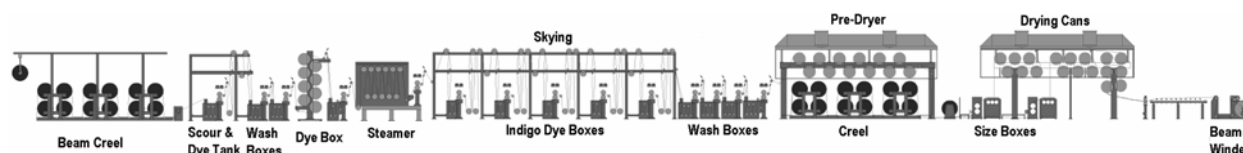
Figure 8. Slasher Indigo Dye Range
