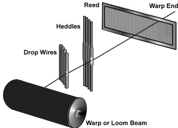
Figure 14. Warp Drawing-in
