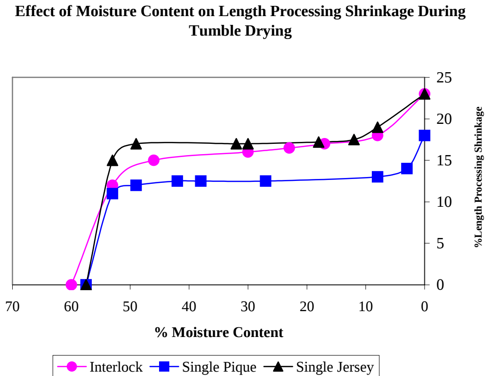
Figure 2: Effect of Moisture on Length Processing Shrinkage
