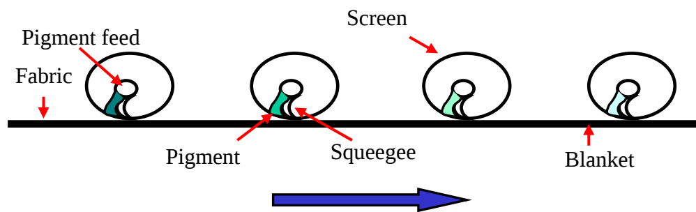
Rotary Screen Printing
