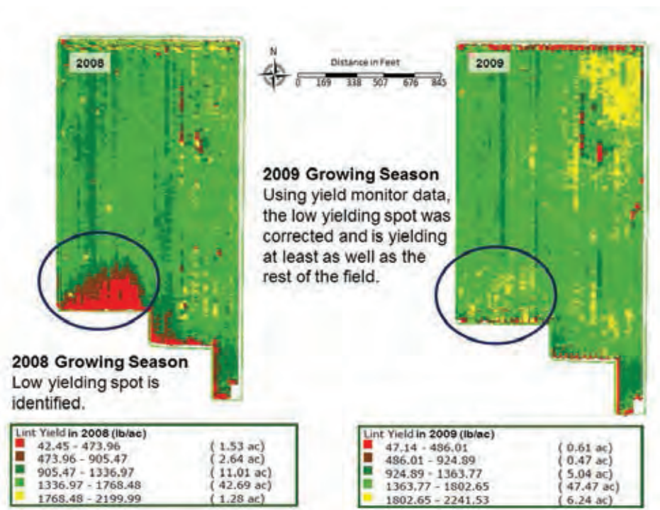
Figure 4: Yield maps of the 63 ac field near Altus, Oklahoma, before and after drain tile was installed to improve yields.
