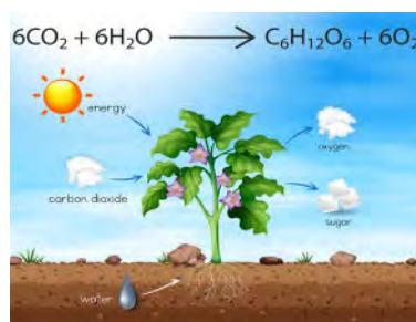
Figure 5. Photosynthesis is a natural way of sequestering atmospheric carbon dioxide into plant material 6
