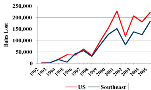
Figure 2. Estimates of cotton bale losses due to stink bug damage, US and Southeast Regions 1992-2005 (Beltwide Cotton Conferences).
