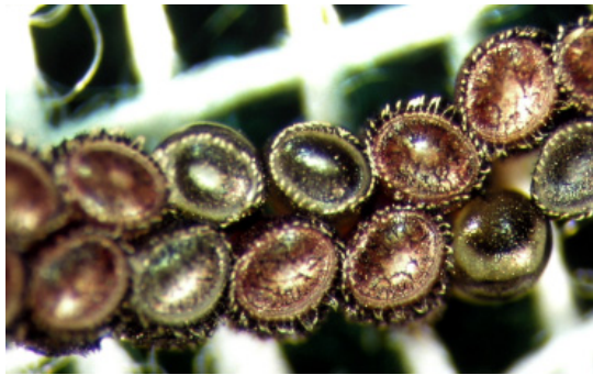
Figure 33. Egg mass of redbanded stink bug.
