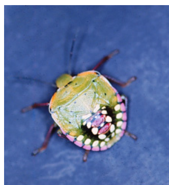
Figure 12. Immature (5th instar) of southern green stink bug.
