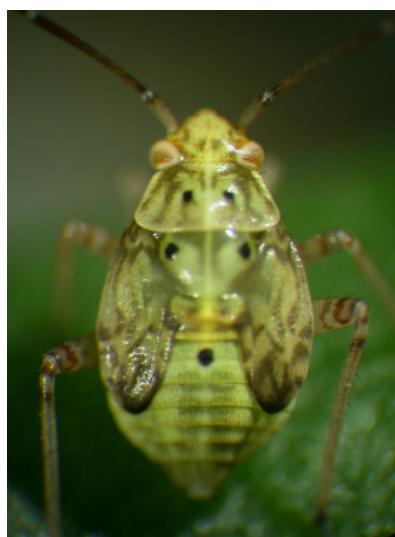
Figure 52. Nymph (5 th instar) of western tarnished plant bug.
