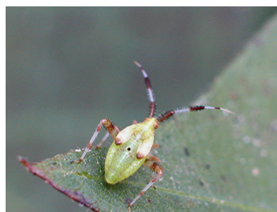
Figure 54. Nymph of clouded plant bug, Neurocolpus nubilus .
