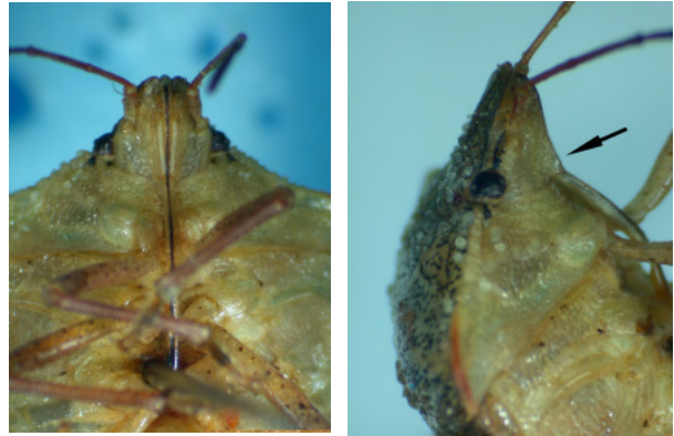
Figure 5. Ventral (left) and lateral (right) views of proboscis of plant-feeding stink bug. Arrow indicates attached first segment of proboscis.
