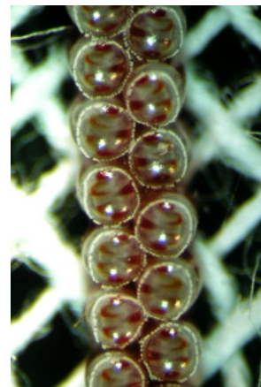
Figure 40. Egg mass of rice stink bug.
