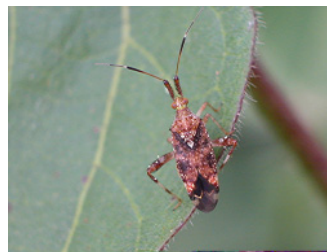
Figure 53. Adult of clouded plant bug, Neurocolpus nubilus .
