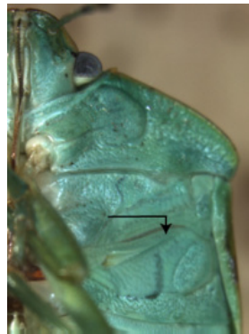
Figure 17. Scent-gland opening of green stink bug. Arrow indicates extension of scent-gland opening more than halfway to margin of thorax.
