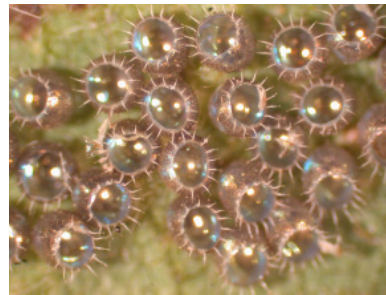
Figure 44. Egg mass of spined soldier bug.
