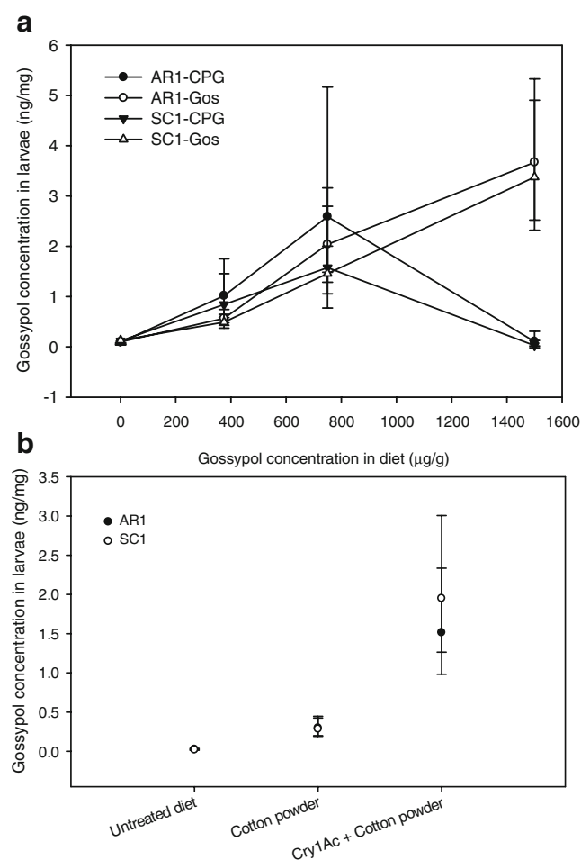
Fig. 3 Concentration of gossypol in Cry1Ac-resistant (AR1) and susceptible (SC1) Helicoverpa zea . When fed on a different concentrations of gossypol (375 μg/g, 750 μg/g & 1,500 μg/g) in the diet alone and in 1:1 combination with Cry1Ac (3.75 μg/g, 7.5 μg/g, 15 μg/g). CPG=Cry1Ac + Gossypol; Gos = Gossypol. b 4% cotton powder alone or in combination with 15 μg Cry1Ac/g diet. The data represent the mean of three replications and standard errors are back-transformed values from logarithmic scale
