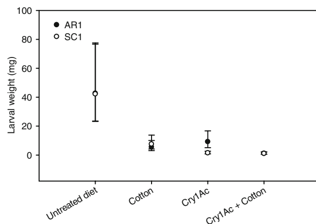
Fig. 4 Effect of 4% cotton powder in the presence and absence of 15 μg Cry1Ac/g diet on larval weight in Cry1Ac-resistant (AR1) and susceptible (SC1) Helicoverpa zea . The data represent the mean of three replications and standard errors are back-transformed values from logarithmic scale
