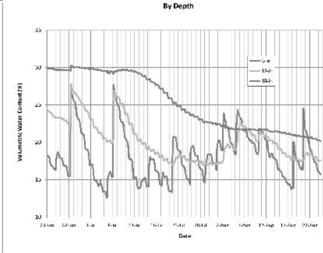
Fig. 1. Graph of average soil moisture % for 6-, 12-, and 18-inch depths for Site 1, 2, and 3. “Bleeding” data has been corrected.
